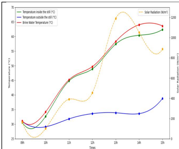
Figure 5: Temperatures inside the distiller, outside the distiller, brine water and solar irradiation as a function of time measured on August 26, 2024
