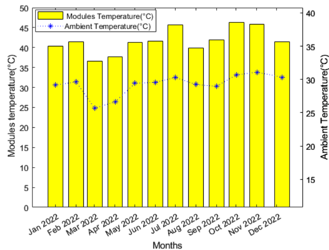
Fig. 4 Monthly variation of ambient temperature and modules
