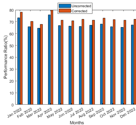
Fig. 6 Temperature-corrected and uncorrected performance ratio
