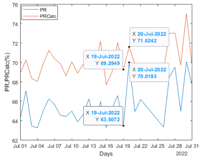
Fig. 8 Correction of performance due to the rain effect
