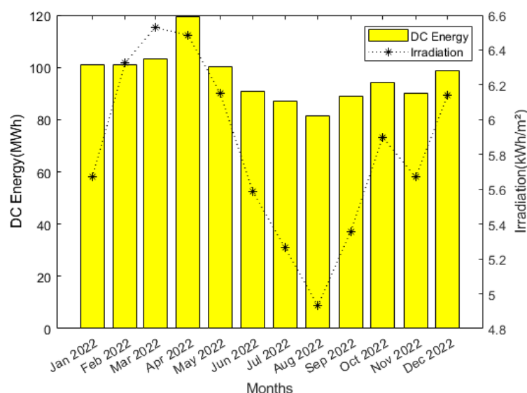
Fig. 2 Monthly variation of daily average energy with irradiation
