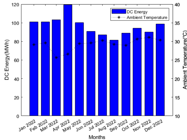
Fig. 5 Monthly variation of daily average energy with temperature
