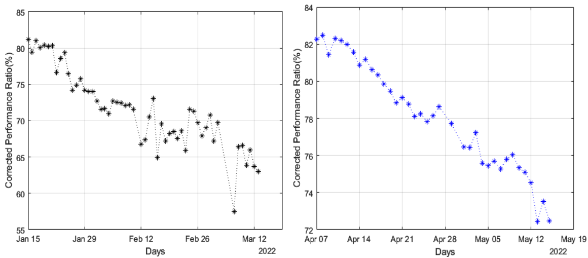
Fig. 7 Performance degradation due to dust
