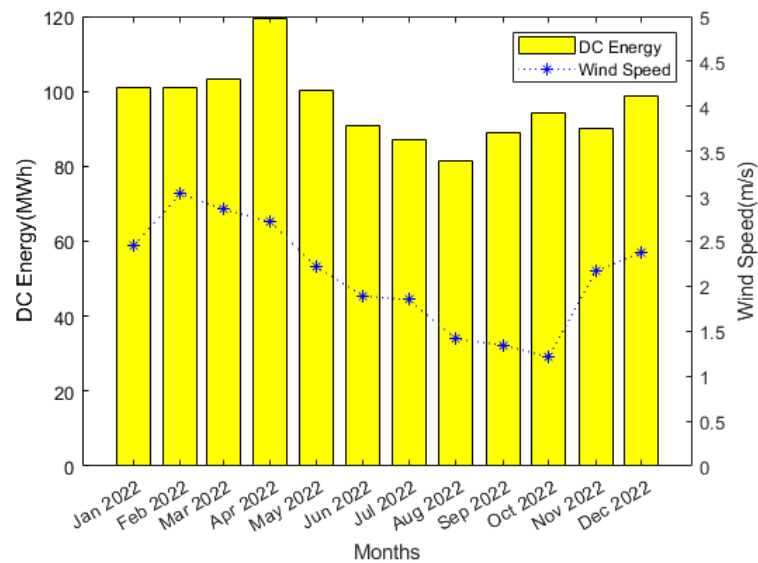
Fig. 3 Monthly variation of daily average energy with wind
