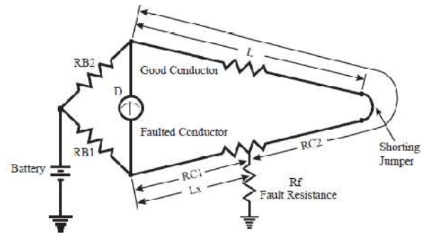
Fig. 3 Murray Loop Bridge application
