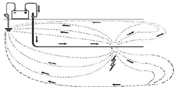
Fig. 1 An A-Frame method of finding cable fault location
