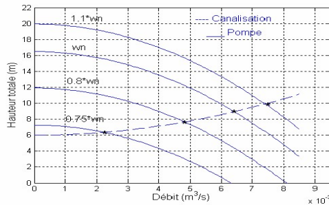
Fig 5.Characteristics H(Q).
