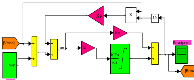
Figure 9. PI regulator loop of voltage.
