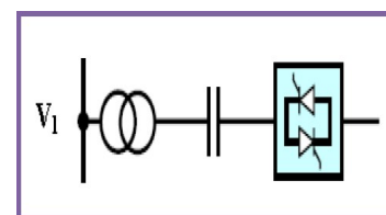
Figure 2. Structure of TSC.
