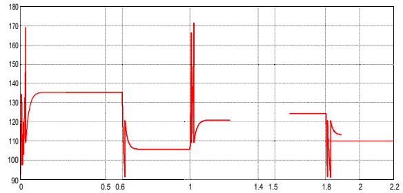
Figure 15. Switching angle ( \alpha ) of TCR.
