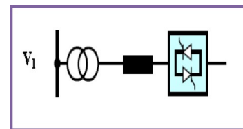
Figure 1. Structure of TCR.
