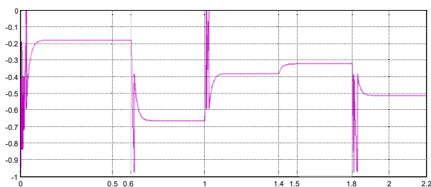
Figure 13. Effective susceptance of TCR (BTCCR).
