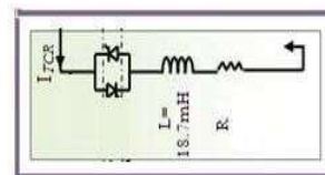
Figure 7. Principal constitution of TCR.
