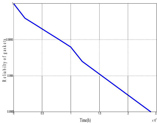
Fig. 6: Gaskets
