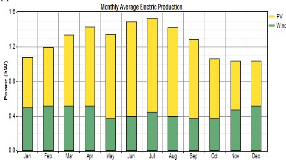
Fig.10 Monthly average electric production
