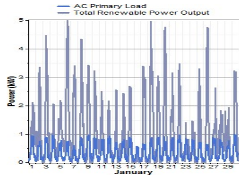
Fig.13 total renewable power produced in January.
