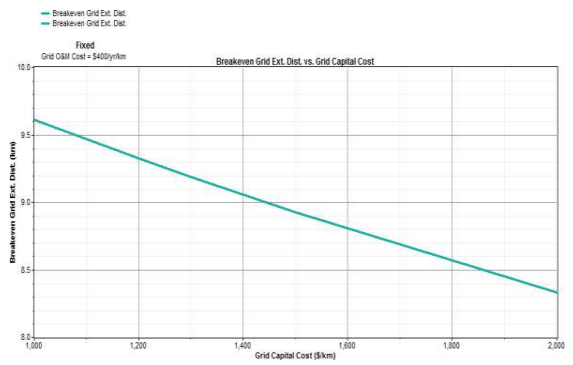
Fig.17 Breakeven grid extension vs. grid capital cost for fixed grid O&M cost=400 $/y/km
