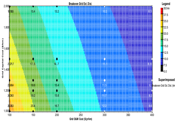
Fig.15 Sensitivity plot for breakeven grid extension
