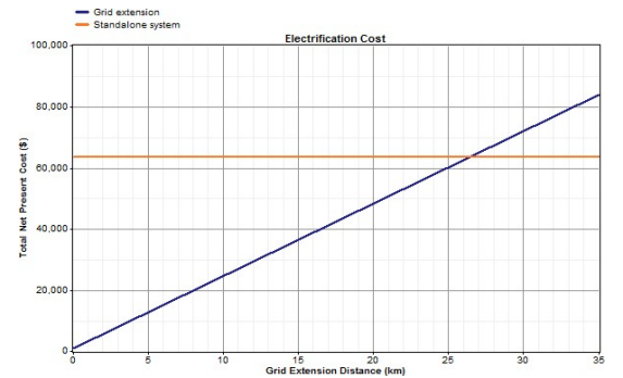
Fig.18 grid extension cost vs. grid extension distance
