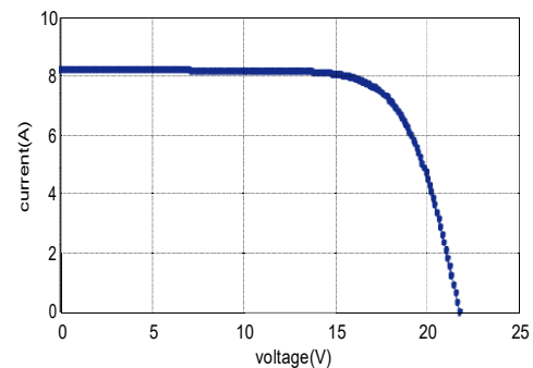
Fig. 2 Suntech STP135-12/Tb I(V) characteristic.
