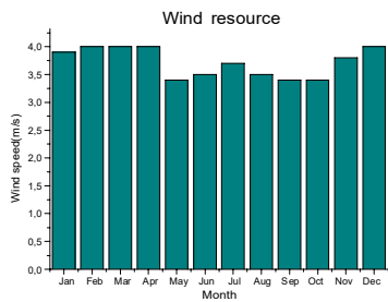
Fig.5 Average annual wind speed in UDES
