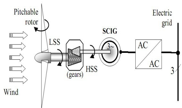
Fig.1 A wind energy conversion scheme
