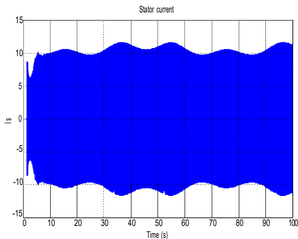
Fig.10 Stator current
