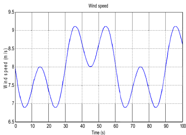
Fig.5 Wind speed
