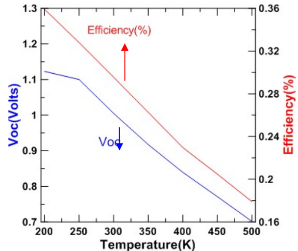
Figure 6. Efficiency and open circuit voltage as a function of temperature for \text{In}_{0.62}\text{Ga}_{0.38}\text{N} SJ solar cell.
