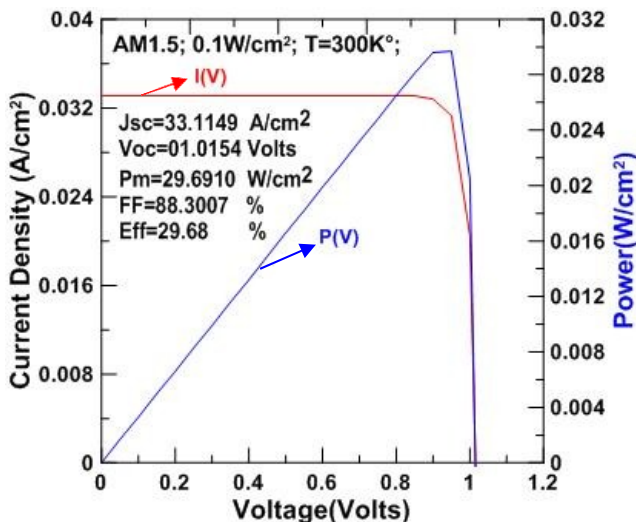
Figure 5. I(V) and P(V) characteristic of the \text{In}_{0.62}\text{Ga}_{0.38}\text{N} SJ solar cell with the optimum performance.
