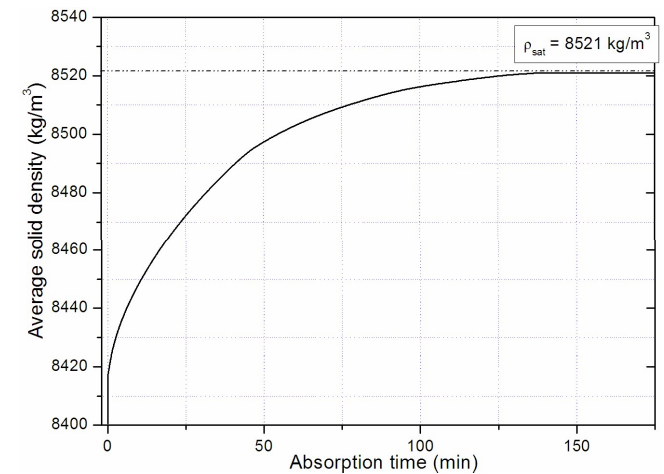
Fig. 5 Averaged solid density evolution.
