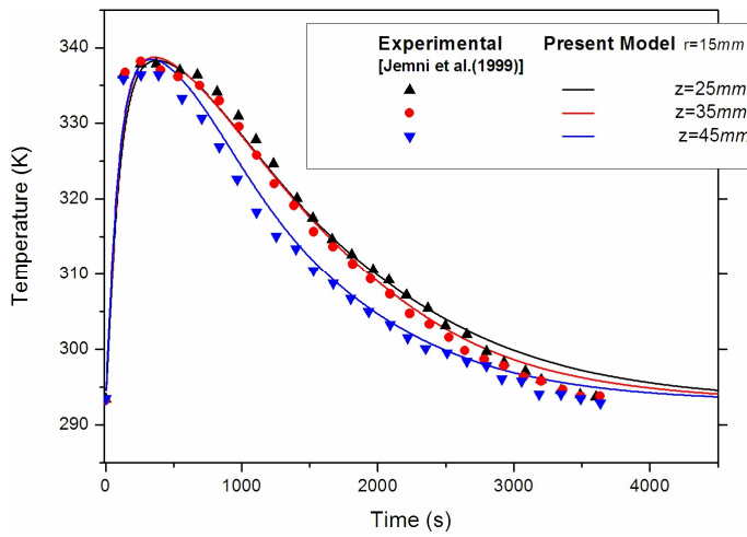
Fig. 2 Temperature evolution at three points within the cylindrical MH tank experimented by Jemni et al. [4] in the hydriding case with the cooling fluid temperature at 20°C.
