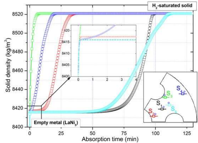
Fig. 4 Solid density history at selected monitoring points.
