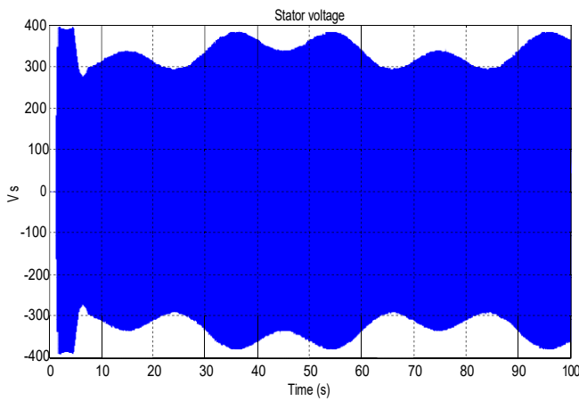
Fig.9 Stator Voltage
