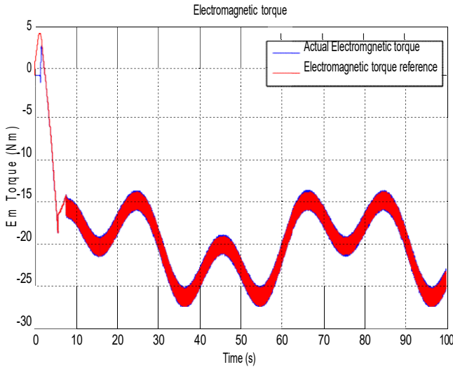
Fig.8 Actual electromagnetic torque and its reference
