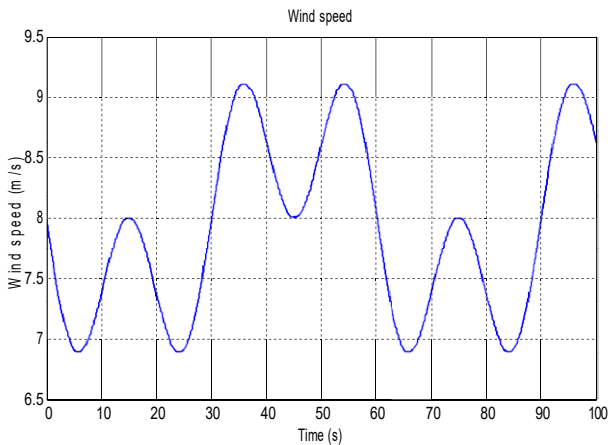
Fig.5 Wind speed
