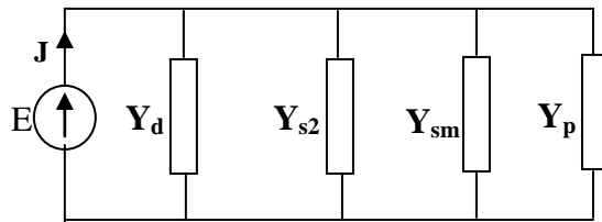
Fig. 3 Equivalent circuit for the structure without target
