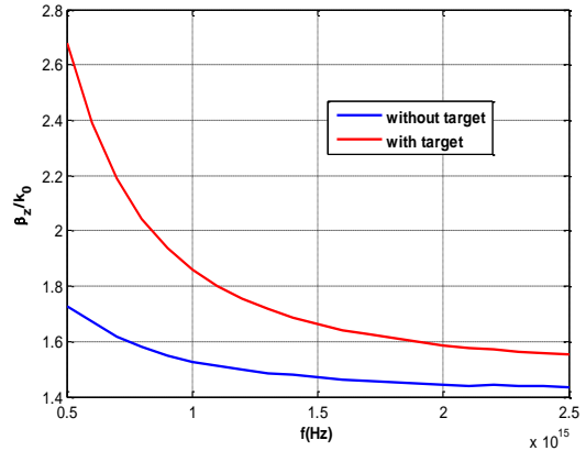
Fig. 6 Dispersion diagrams for TM Surface Plasmon mode of our structure without and with the layer illustrated the target.
