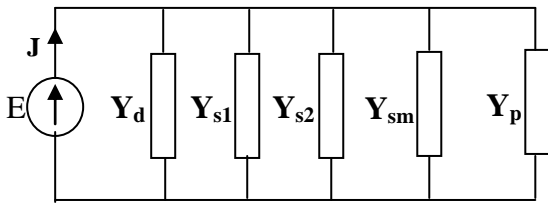
Fig. 4 Equivalent circuit for the structure with target
