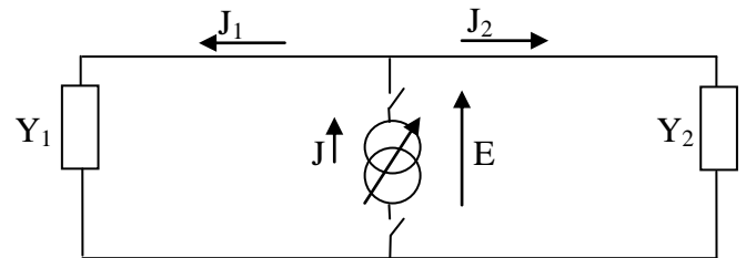
Fig. 2 Equivalent circuit used to illustrate the Transverse Resonance Method
