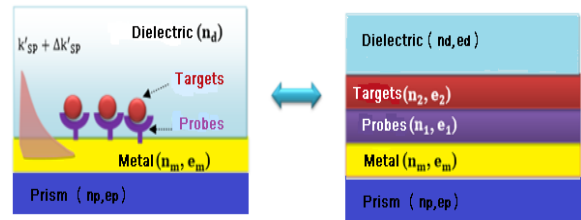
Fig. 1 Equivalent structure to the principle of a perturbation generated by a biomolecular interaction on the surface of a Surface Plasmon biochip
