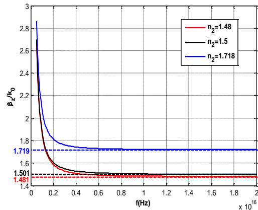
Fig. 7 Normalized real constant of TM Surface Plasmon mode propagating at surface of metal versus frequency for different targets detected
