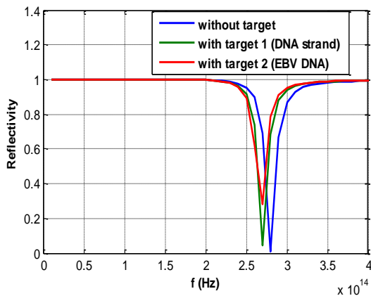
Fig. 8 Spectral shift caused by the deposition of target layer on the metal surface
