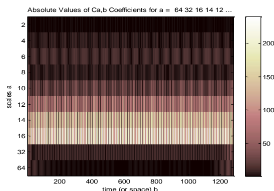
Fig. 12 Scalogram of CWT of the system degraded motor - reducer following an unbalance
