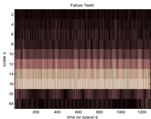
Fig. 15 CWT scalogram of the Faulty system motor-reducer due to wear of 3 teeth
