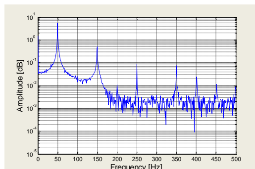
Fig. 6 FFT of healthy system
