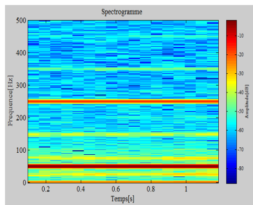
Fig. 7 STFT of healthy system
