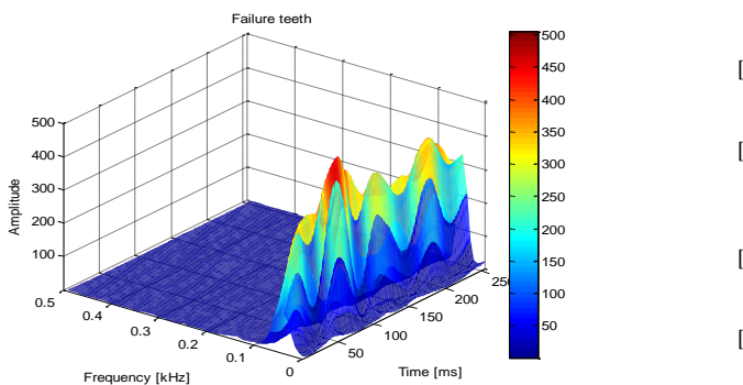
Fig. 14 Gabor spectrogram of the Faulty system motor-reducer due to wear of 3 teeth
