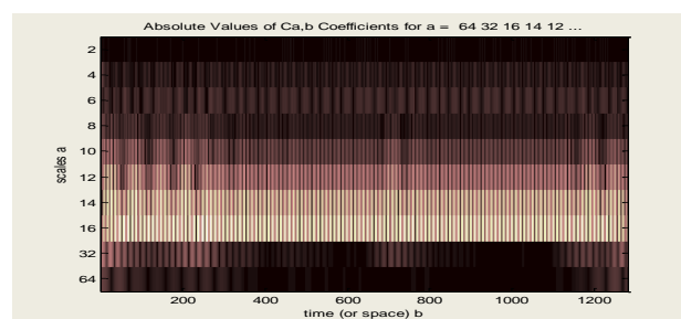
Fig. 9 CWT of healthy system
