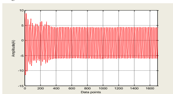
Fig. 5 Time significance of the stator current
