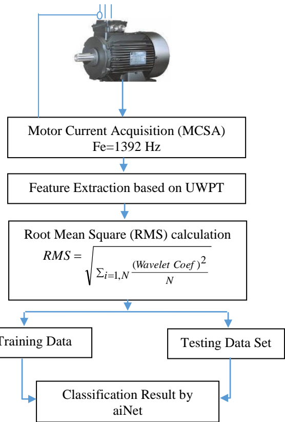
Fig.7. Fault Diagnosis Algorithm
