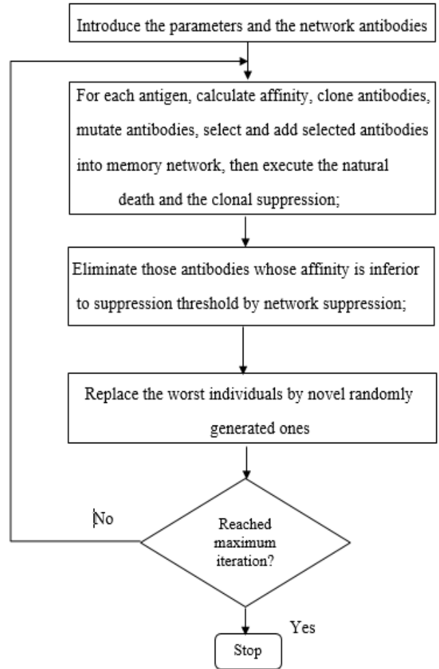
Fig.2. The procedure of aiNet algorithm.
