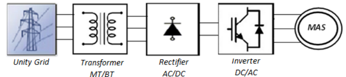
Fig 1. Chain constituting
