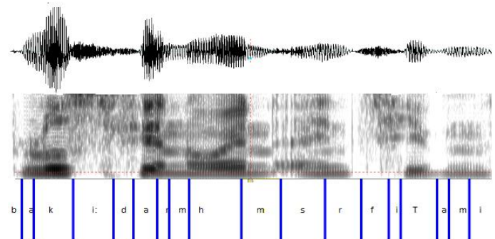
Fig 5 Example MAUS segmentation and labeling taken from the Arabic corpus with SAMPA code.
