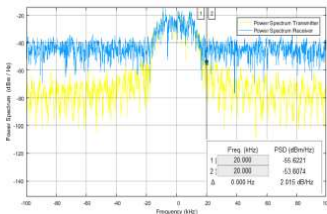
Figure (5) Transmit and Receive Spectra at the carrier frequency of 12000 MHz
