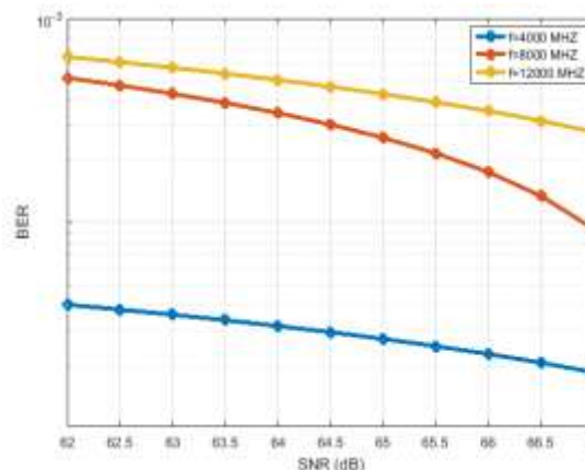
Figure.(8) The Relationship Between Bit Error rate and the SNR(dB)
