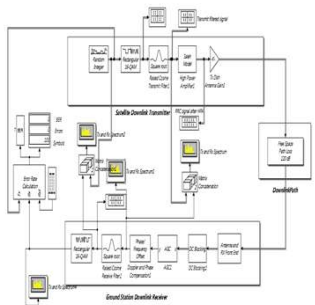
Figure (2) Simulation Model of RF Satellite downlink of the C band, so it is possible to build a receiver system.
