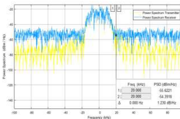
Figure (3) Transmit and Receive Spectra at the carrier frequency of 4000 MHz
