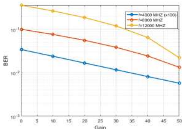
Figure.(6) The Relationship Between Bit Error rate and the Gain
