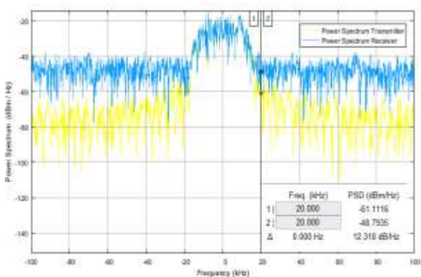
Figure (4) Transmit and Receive Spectra at the carrier frequency of 8000 MHz
