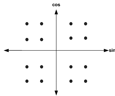
Figure (1)the constellation diagram of 16 QAM
