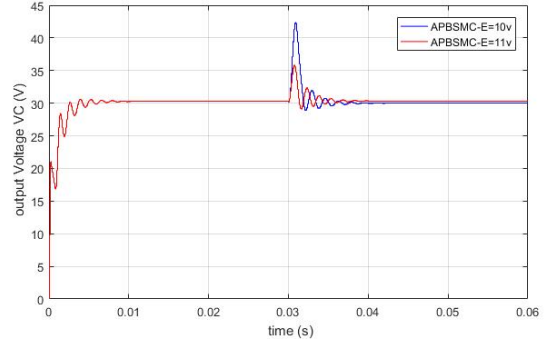
Fig. 11. Output voltage response v_C with source E perturbations (APBSMC approach).
