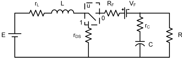
Fig. 1. Circuit equivalent of a boost converter with parasitic parameters.
