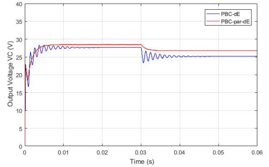
Fig. 7. Output voltage response v_C with Source E perturbation for PBC and PBC-par control laws.
