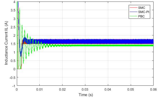
Fig. 2. Inductance current i_L for approaches (SMC, cascaded SMCPI and PBC).
