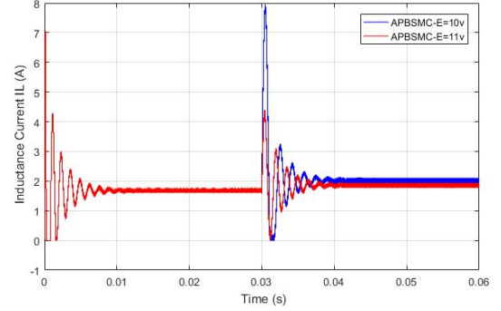
Fig. 10. Inductance current i_L with source E perturbations (APBSMC approach).
