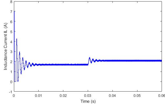
Fig. 8. Inductance current i_L with load variation (APBSMC approach).
