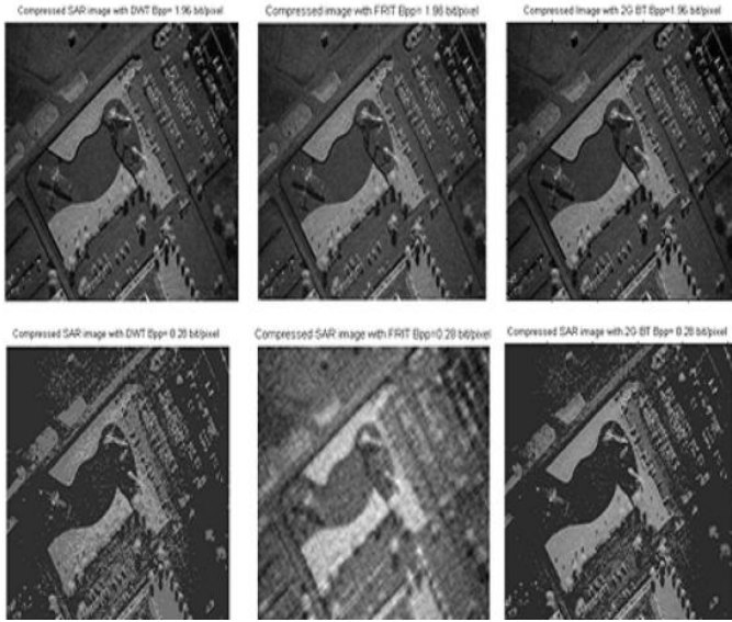
Fig. 6 Comparison of SAR image compression, at \text{bpp}=1.96 bit/pixel (DWT PSNR =35.86 dB, FRIT PSNR = 34.71 dB and 2GBandelet PSNR = 37.18dB) and at \text{bpp}=0.28 bit/pixel (DWT PSNR =19.55 dB, FRIT PSNR = 18.85 dB and 2G Bandelet PSNR = 24.10dB)
