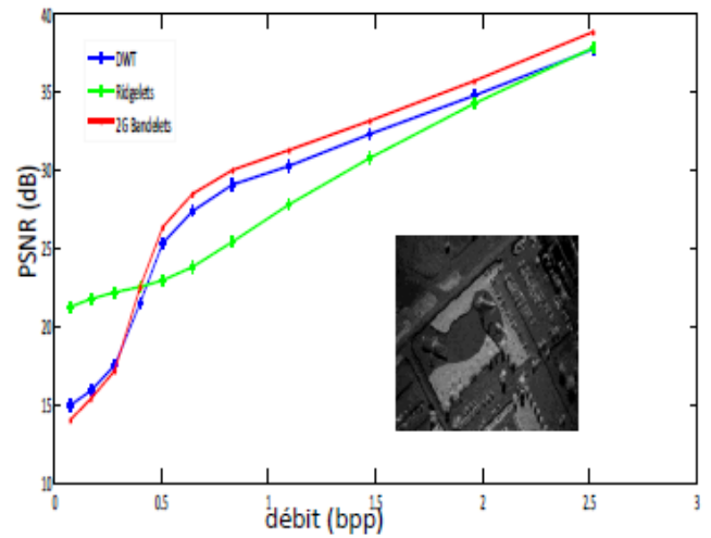
Fig. 8 Result of SAR image compression using 2G bandelet, Wavelet and FRIT transforms
