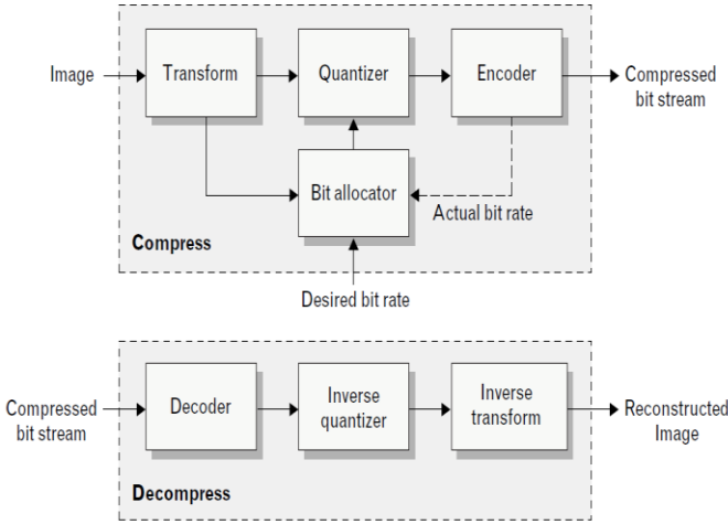
Fig. 5 Scheme of compression system based on the transform [1]
