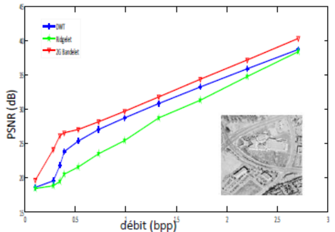
Fig. 9 Result of Aerial image compression using 2G bandelet, Wavelet and FRIT transforms
