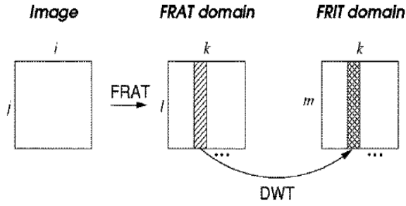
Fig. 4 The Finite Ridgelet Transform [8]
