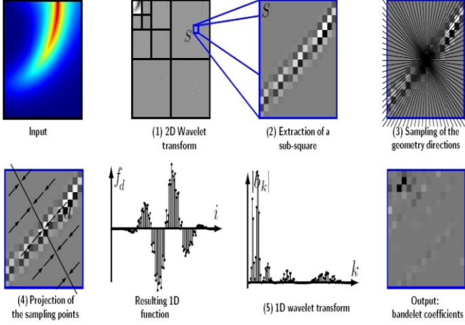
Fig. 3 Framework of the second generation of bandelets transform[2]
