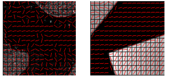
Fig. 2 Geometric flow under different dyadic square segmentation
