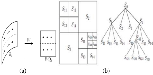
Fig. 1 (a) Example of deformation W of a region \Omega_i , (b) Quadtree decomposition [2,3]
