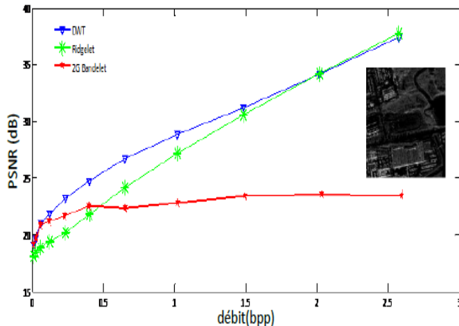
Fig. 10 Result of SABR Radar SAR image compression using 2G bandelet, Wavelet and FRIT transforms
