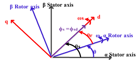
Fig.3 Flux orientation
