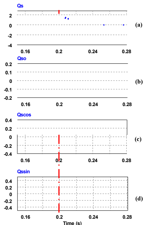
Fig.6 Reactive power for DFIG faulty operation
