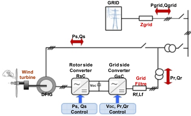
Fig.1 Variable speed wind system based on DFIG
