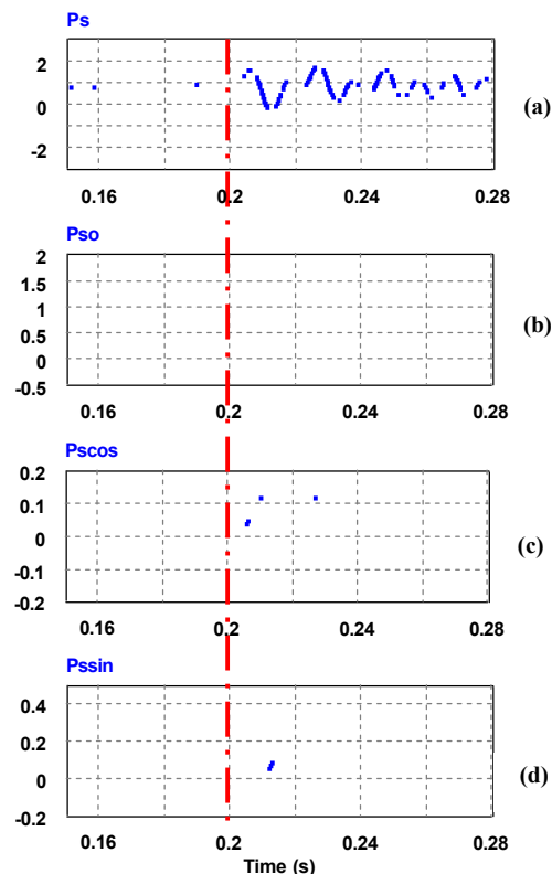
Fig.5 Active power for DFIG faulty operation
