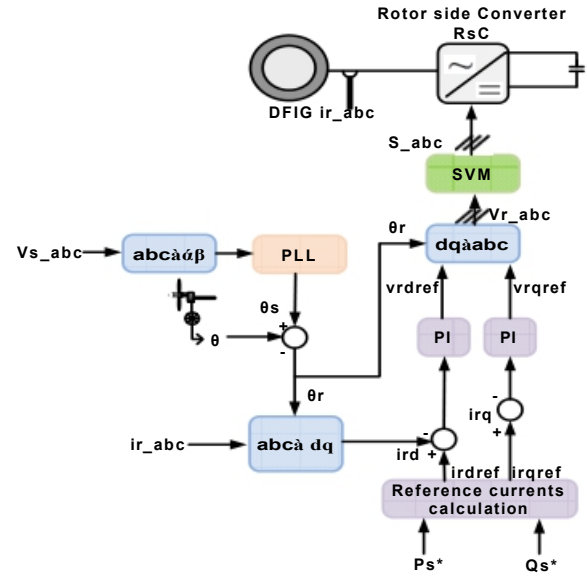
Fig.2 RsC proposed control
