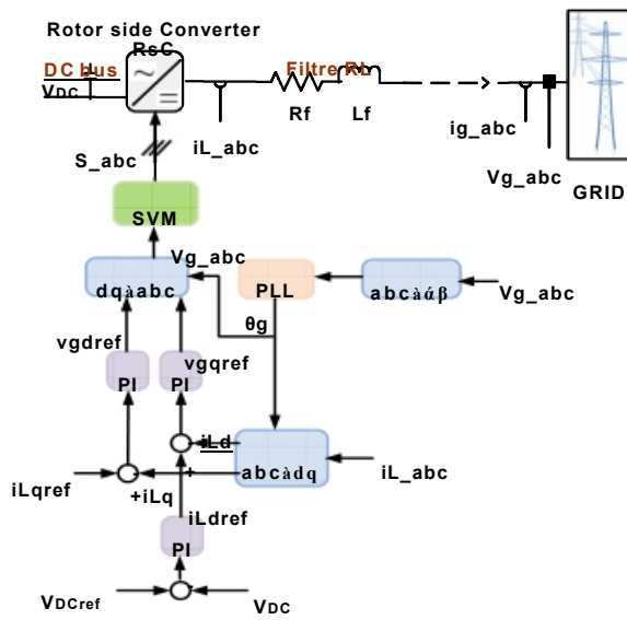
Fig.4 GSC proposed control
