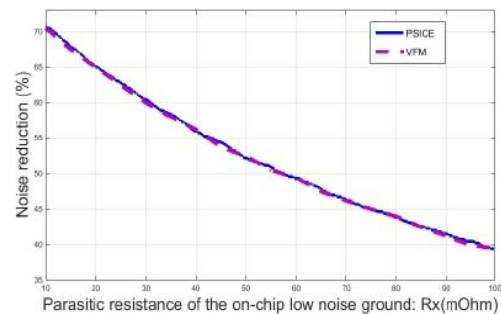
Fig. 7. The noise reduction for different values of the parasitic resistance of the ground plane
