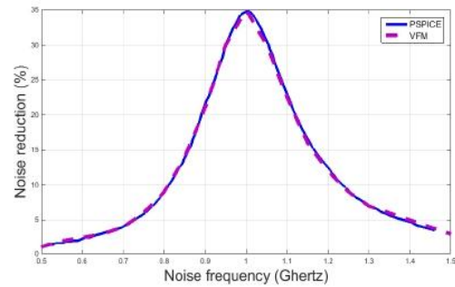
Fig. 5. The noise reduction for a sinusoidal noise source according to the frequency
