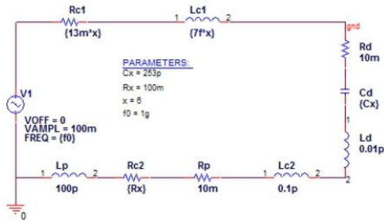
Fig. 3. The equivalent circuit of the noise reduction technique (ground plane)
