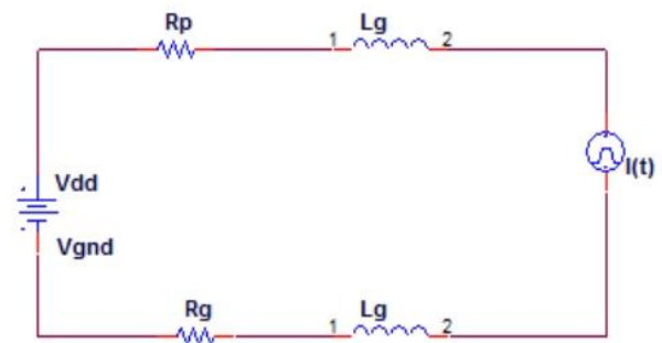
Fig. 1. The equivalent circuit of a basic power supply network
