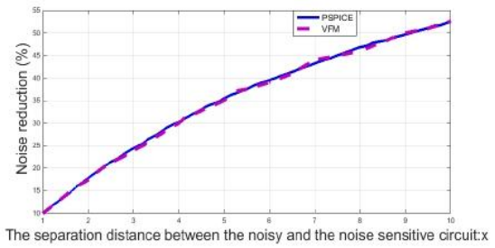
Fig. 4. The reduction of noise versus the separation distance between the circuit aggressors and the circuit victims
