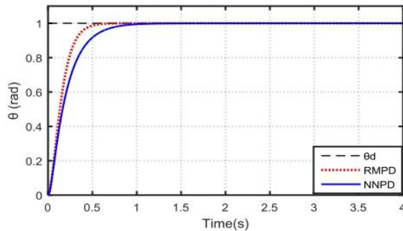
Fig.6 Step response of pitch angle
