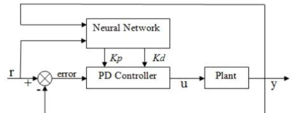
Fig.2 Structure of PD Control System Based on Neural Network
