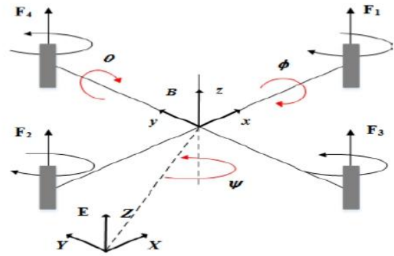
Fig.1 Quadcopter Configuration
