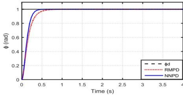
Fig.5 Step response of roll angle
