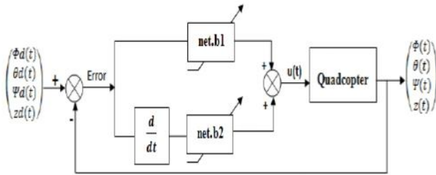
Fig. 4. Structure of the neuronal PD control
