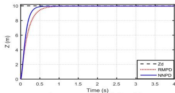
Fig.8 Step response of altitude position
