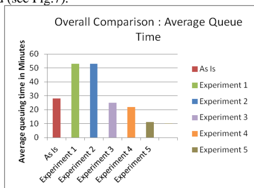
Fig.7. Overall Comparison, average queue time
