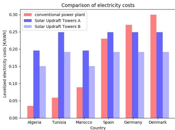
Fig. 5 Comparison of electricity cost.
