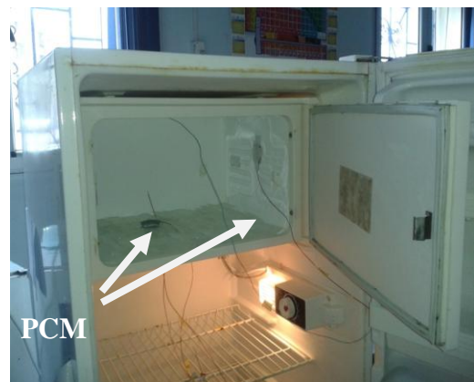
Fig.3 PCM integrated in contact with evaporator
