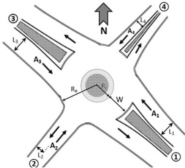
Fig. 2 Geometry layout of the studied intersection
