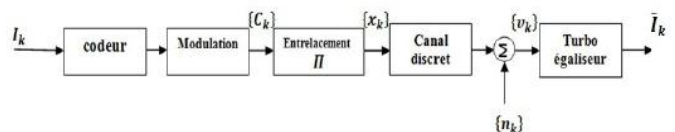
Fig.2 Communication chain with a turbo equalizer.
