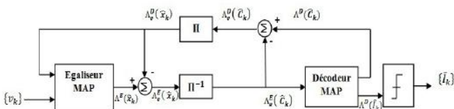
Fig.5 Operating principle of the MAP turbo equalizer - MAP.
