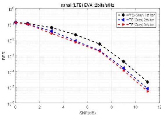
Fig.8 TE performance (AI, decoder-TCM) for different iteration processes.
