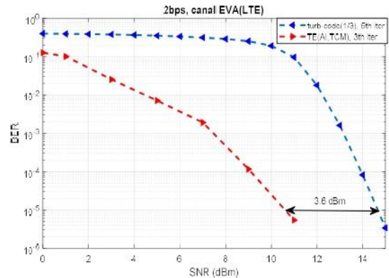
Fig.9 Comparison of the transmission performance of LTE system that uses a simple ZF equalizer, and the LTE system that uses turbo-equalizer (AI, TCM decoder), in the EVA channel.
