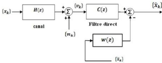
Fig.1 Interference cancelling equalizer (AI).
