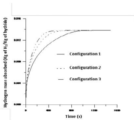
Fig.5 Time evolution of the hydrogen mass absorbed for the three configurations
