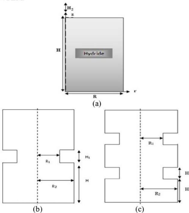
Fig. 1 Various designs of reactors studied: (a) basic reactor (configuration 1), (b) modified MHR (configuration 2), (c) modified MHR (configuration 3)
