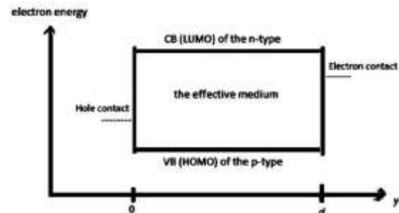
Fig.2 Schema of the effective medium model (EMM).
