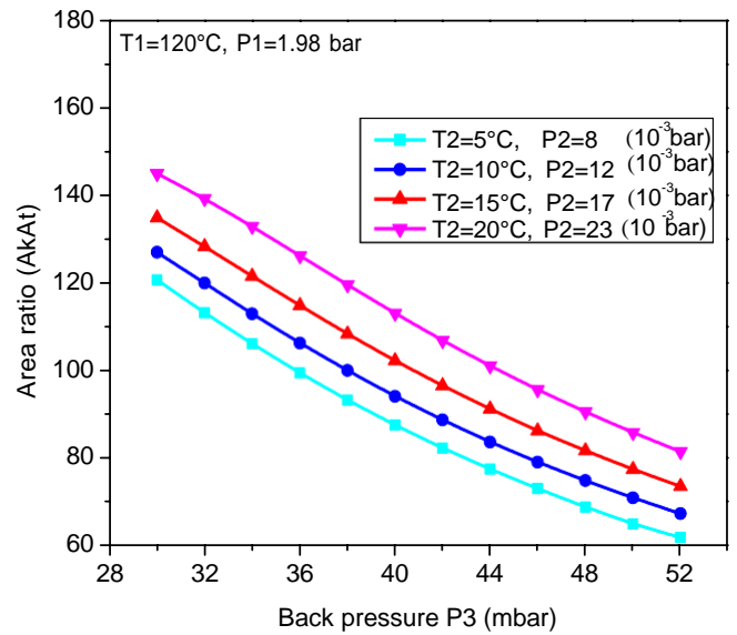
Fig. 5. Effect of back Pressure on Ejector Area Ratio.
