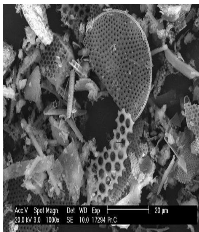
Fig. 4 SEM micrograph of the diatomite powder
