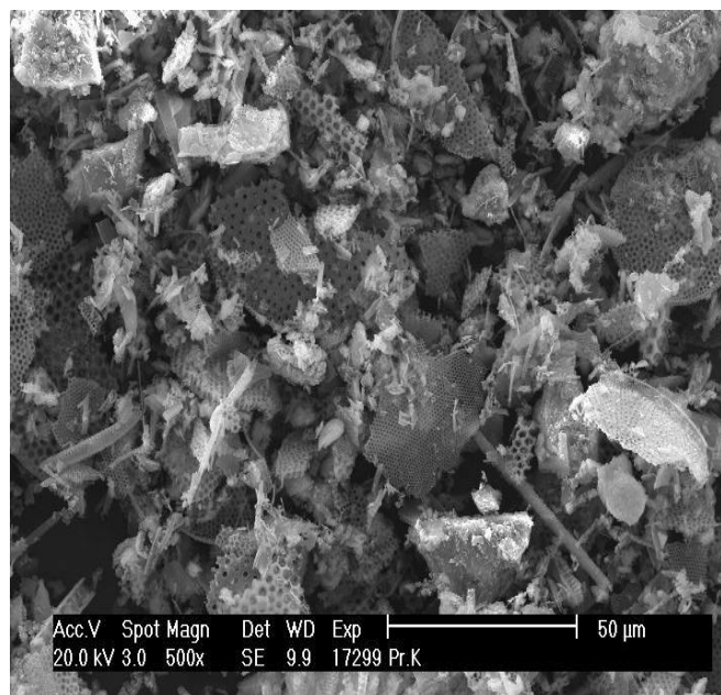
Fig. 3 SEM micrograph of the diatomite powder
