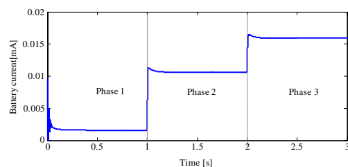
Figure 12 . Variation of battery current in different phases.
