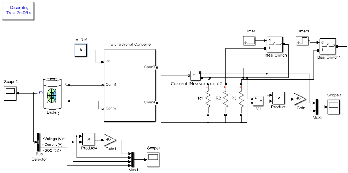
Figure 9. Model of wireless sensor Networks in MATLAB/Simulink.
