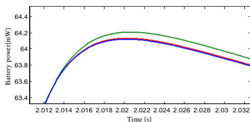
Figure 21. Comparative of peak power in different battery technologies at the end of transmission phases.
