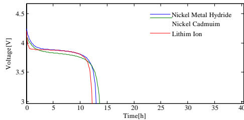
Figure 25. Discharge curve for 200 mA current.
