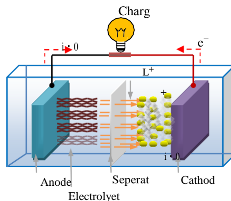
Figure 3. Diagram of charged lithium-ion battery.
