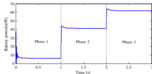
Figure 11. Variation of battery power in different phases
