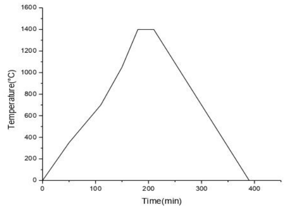
Fig. 3 Thermal cycle of mortar specimens
