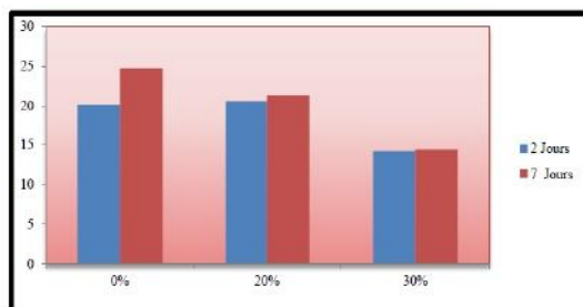
Fig. 7 Compression test results by substituting normalized sand with bentonite
