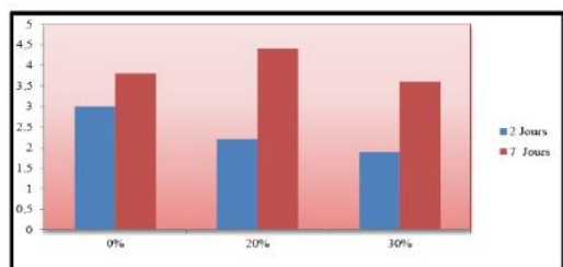
Fig. 6 Results of flexural tests by substituting normalized sand with bentonite
