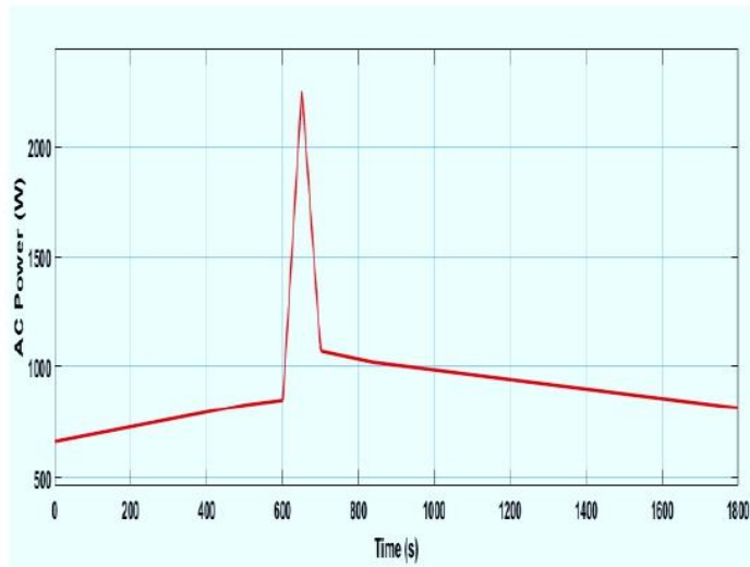
Fig 4 AC Power with DC-AC converter Efficiency is 98%
