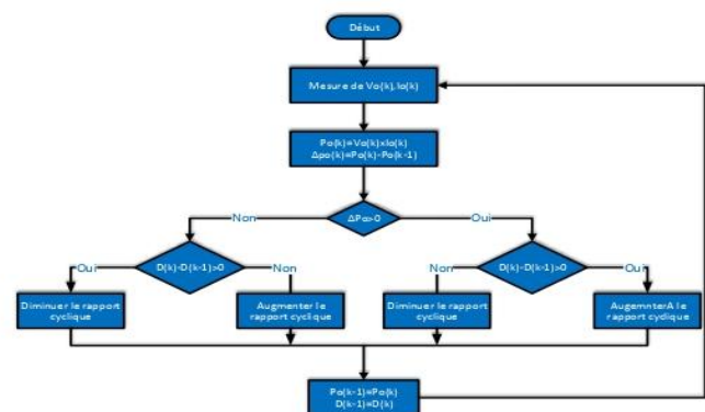
Fig. 3 Flowchart of P&O Algorithm for MPPT control
