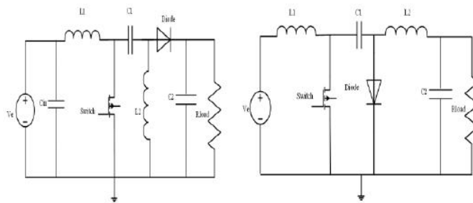
Fig. 5 Circuit diagram of SEPIC converter
