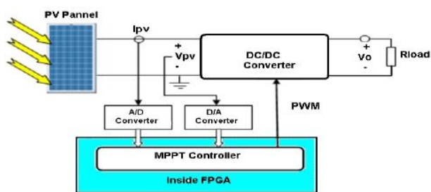
Fig. 14 Diagram of the principle of the adopted PV system with integrated controller on FPGA
