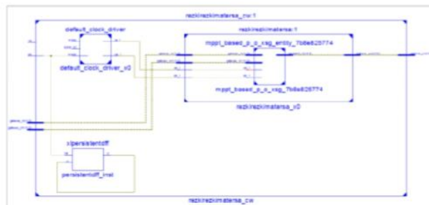
Fig. 15 Global RTL scheme of the P & O algorithm
