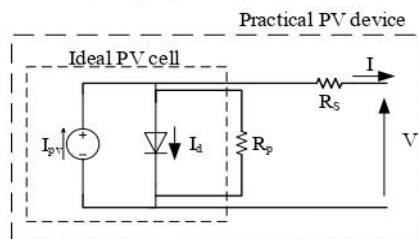
Fig. 1 Circuit equivalent to a single diode of a PV cell
