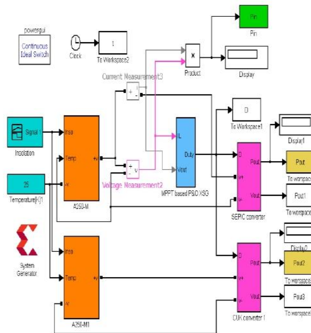
Fig. 6 General architecture of system simulation
