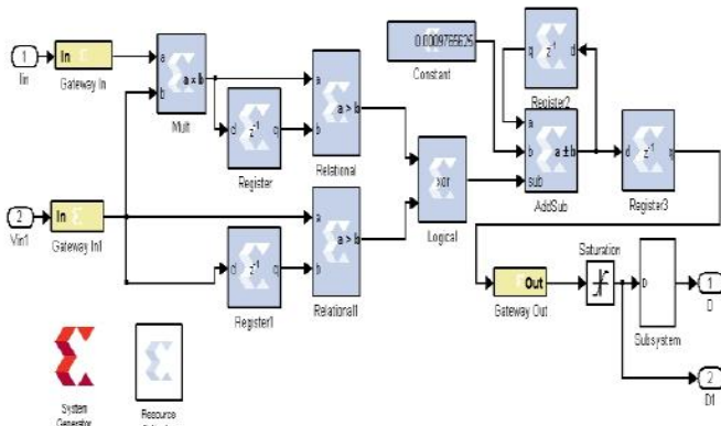
Fig. 7 Implementation of the P&O algorithm based XSG
