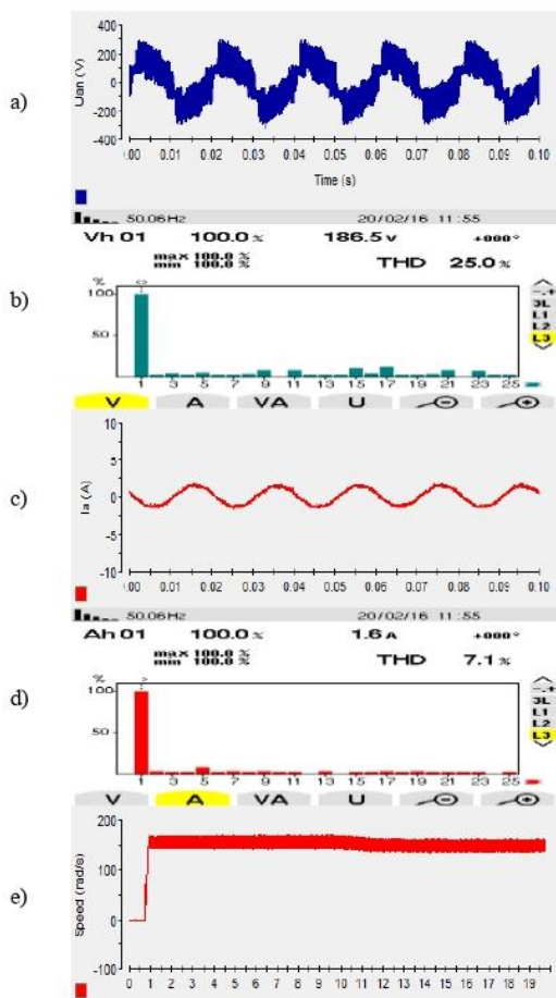
Fig.7. Discontinuous Pulse Width Modulation DPWM_3, M = 0.9 , a)Line to neutral voltage V_m(v) , b)Voltage frequency spectrum THD (%), c) Phase current I_a(A) , d) Current frequency spectrum THD (%) and e) Motor speed (rad/s)
