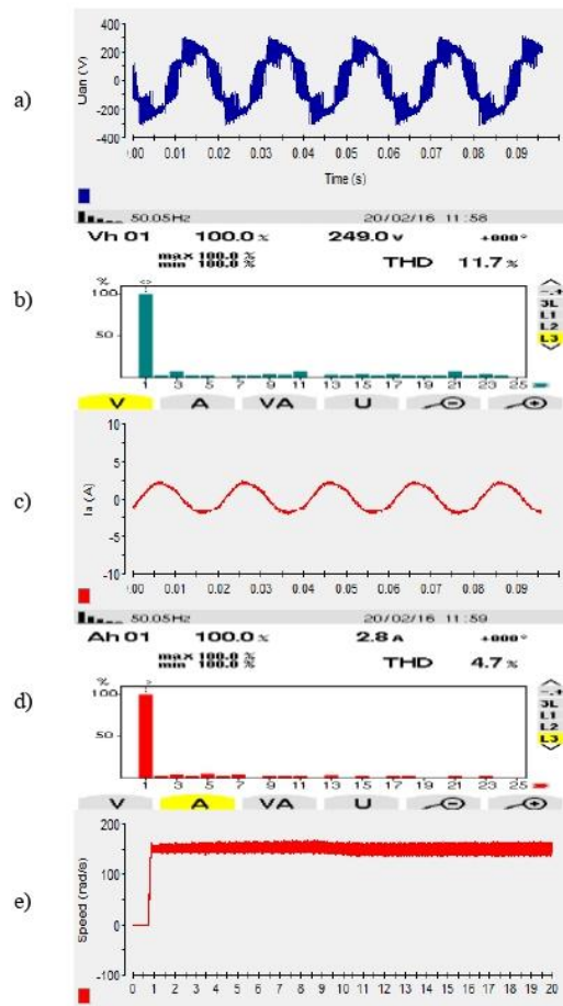
Fig.8. Discontinuous Pulse Width Modulation DPWM_3, M = 1.2 , a)Line to neutral voltage V_m(v) , b)Voltage frequency spectrum THD (%), c) Phase current I_a(A) , d) Current frequency spectrum THD (%) and e) Motor speed (rad/s)
