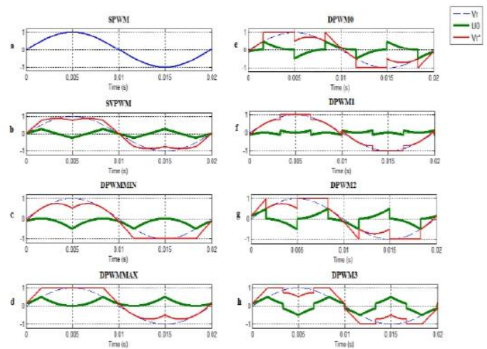
Fig.1. The reference waveforms V_r , V_r^* and the zero-sequence components U_0 injected width different strategies
