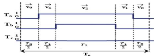
Fig.3. Chronogram of pulses based on two phase PWM (DPWM)
