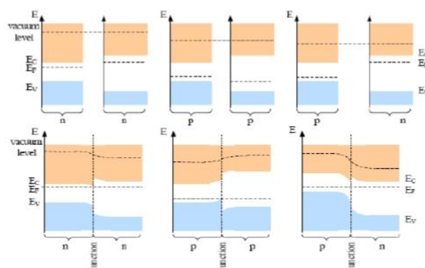
Fig 1 : Band diagram of heterojunction formation[2].
