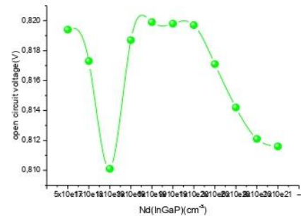
Fig5. Effects of the emitter doping concentration on the open circuit voltage of the solar cell.
