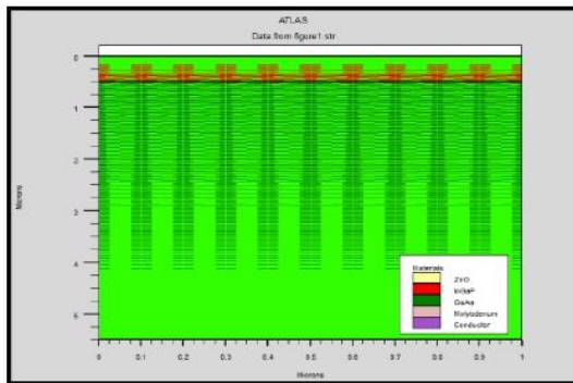
Fig4. Mesh structure of the model.
