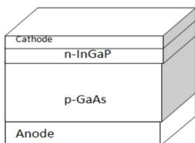
Fig 2 – Schematic representation of the sample structure.
