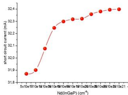
Fig5. Effects of the emitter doping concentration on the short circuit current of the solar cell.
