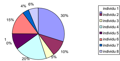
Fig. 7 Proportional roulette
