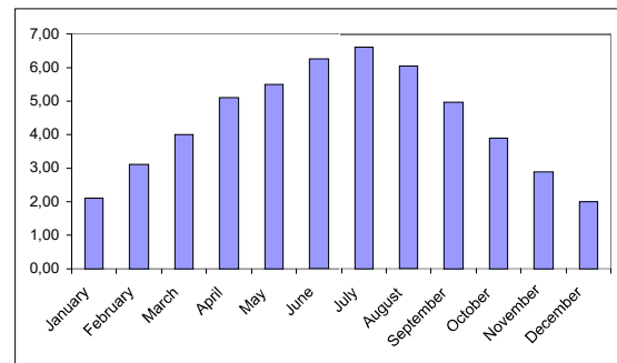
Fig. 2 Irradiation (kWh / m 2 / d) during 2010 in Bejaia.
