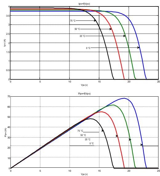
Fig.5 Simulink model I-V and P-V curves which is influenced by cell temperature when the insolation is constant at 1000 W/m 2
