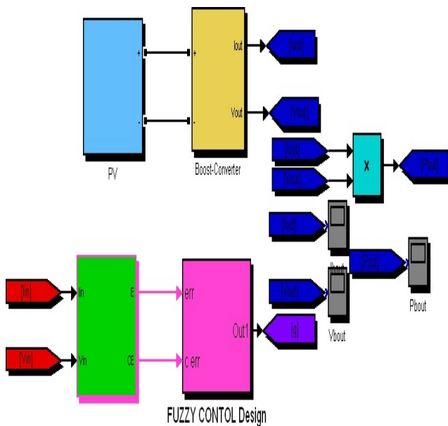
Fig.14 Block simulation of Boost converter with Mppt Fuzzy Control Design
