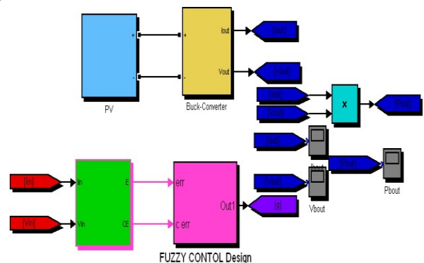
Fig.12 Block simulation of Buck converter with mpp Fuzzy Control Design
