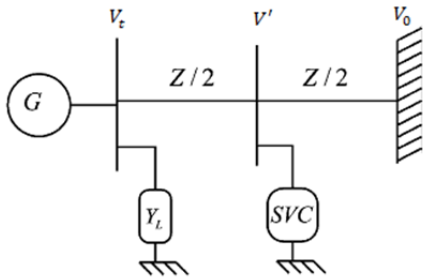
Fig. 1 Single machine infinite bus system with SVC
