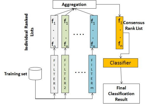
Fig. 2. Feature Selector Based Aggregation
