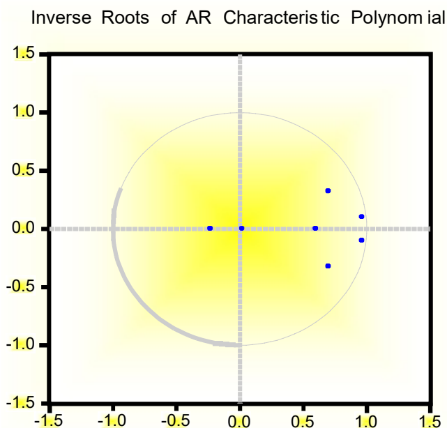
Fig 4. Model Stationarity
